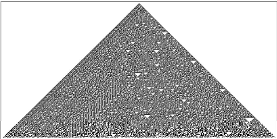
rule 30
